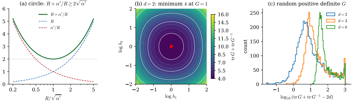
Figure 6: The dual-scale bound. (a) On a circle the effective scale R + \alpha'/R is minimized at the self-dual radius. (b) For d = 2 and positive-definite G with eigenvalues \lambda_{1,2} , \text{tr } G + \text{tr } G^{-1} = \sum_i (\lambda_i + \lambda_i^{-1}) has its minimum 2d = 4 at G = 1 . (c) Excess over 2d for 4000 random positive definite matrices in each dimension: never negative, as the Lean theorem dualScale_ge guarantees. The plot illustrates the theorem; it proves nothing. Computed figure; data: Lean dualScale_circle, circle_effective_scale_ge_two, dualScale_ge (TraceBound.lean).
