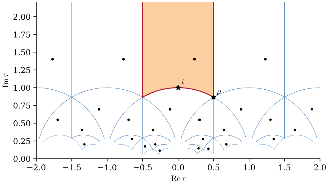
SL(2, \mathbb{Z}) images of the fundamental domain and an orbit of \tau
