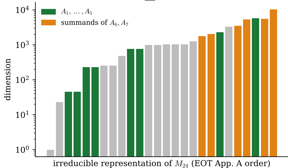
(b) the 26 irreps; \sum \dim^2 = 244\,823\,040 = |M_{24}|
