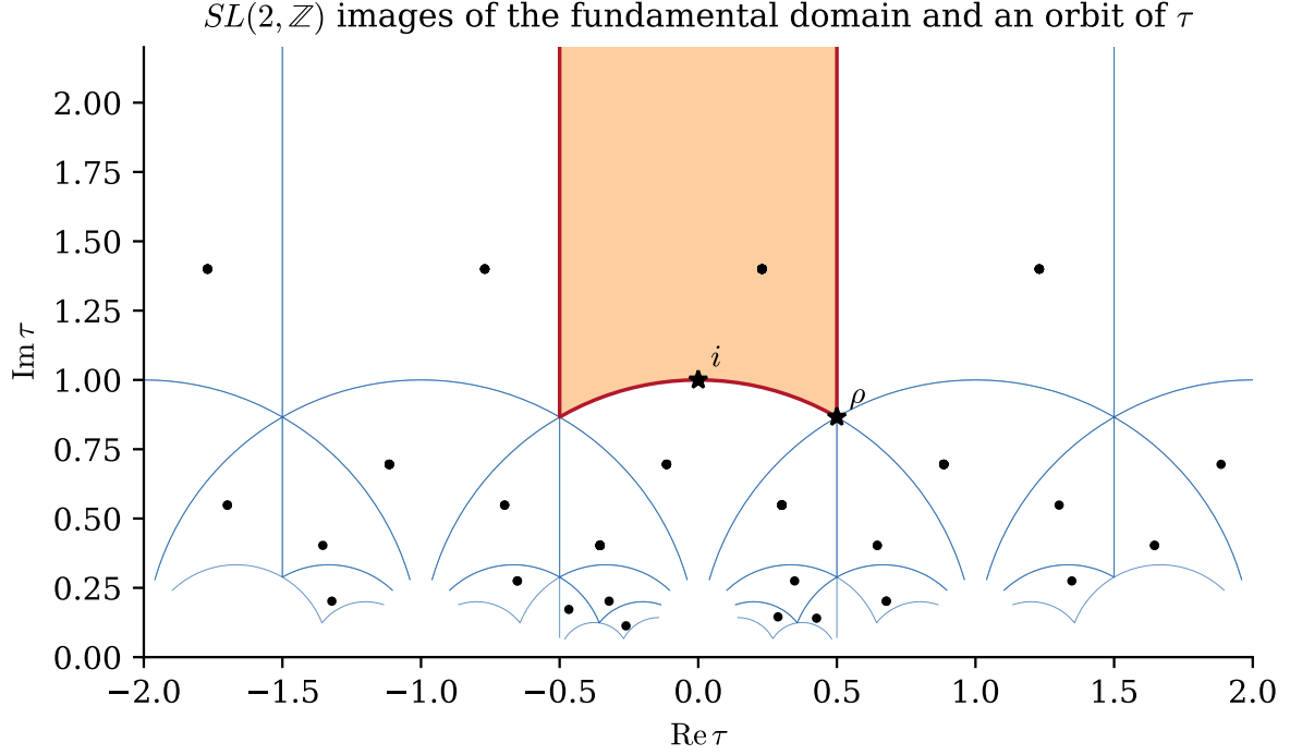
Figure 4: The standard fundamental domain of SL(2, \mathbb{Z}) (shaded) and its images under words of length \leq 4 in S : \tau \mapsto -1/\tau and T : \tau \mapsto \tau + 1 , together with the orbit of one point. For T^2 the same picture holds for both moduli \tau and \rho , exchanged by mirror symmetry. Computed figure; data: GPR §2.5 / Tong §6 (modular group); Lean tauShift , mirror_conjugates_tauShift .
