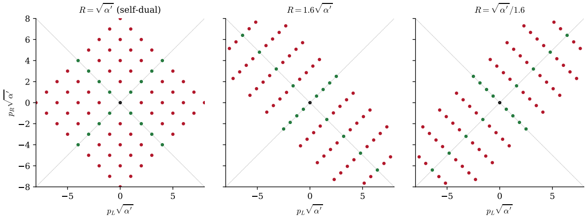
Figure 3: The Narain lattice \Gamma^{1,1} of zero-mode momenta (p_L, p_R) for |n|, |w| \leq 4 at three radii. Changing R is a Lorentz boost in the (p_L, p_R) plane that preserves p_L^2 - p_R^2 = 4nw (dotted light-cone lines); the lattices at R and \alpha'/R coincide after p_R \mapsto -p_R — T-duality. Computed figure; data: Lean leftMomentum , rightMomentum ; GPR §2.3; Tong §8.2.
