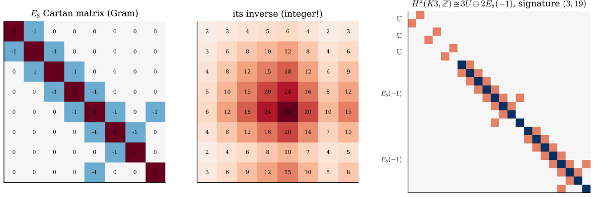
Figure 1: Left: the Gram matrix of E_8 (the Cartan matrix used in Lean) and its inverse, which has integer entries because \det = 1 (unimodularity). Right: the 22 \times 22 Gram matrix of the K3 lattice 3U \oplus 2E_8(-1) (red +, blue -); even diagonal, determinant \pm 1 , signature (3, 19). Computed figure; data: Lean cartanE8 ( E8.lean ), hyperbolicU ( Hyperbolic.lean ); cartanE8Inv_mul , sigK3_eq .
