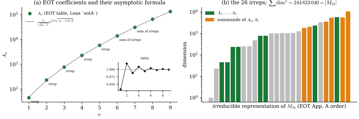
Figure 8: (a) The coefficients A_n of the K3 elliptic genus (EOT eq. 1.12, the Lean table eotA ) against the asymptotic formula EOT eq. (1.13); the inset shows the ratio. A_1, \dots, A_5 are dimensions of irreducible representations of M_{24} ; A_6 and A_7 are sums of them. (b) The 26 irreducible dimensions of M_{24} from the Lean table M24RepDim ; the sum of their squares equals the group order ( M24RepDim_sum_sq ), the check that caught an earlier wrong table. Computed figure; data: EOT eqs. (1.12)–(1.15), ll. 200–232 (formula read from the PDF page, the .txt garbles it); App. A (A.3).
