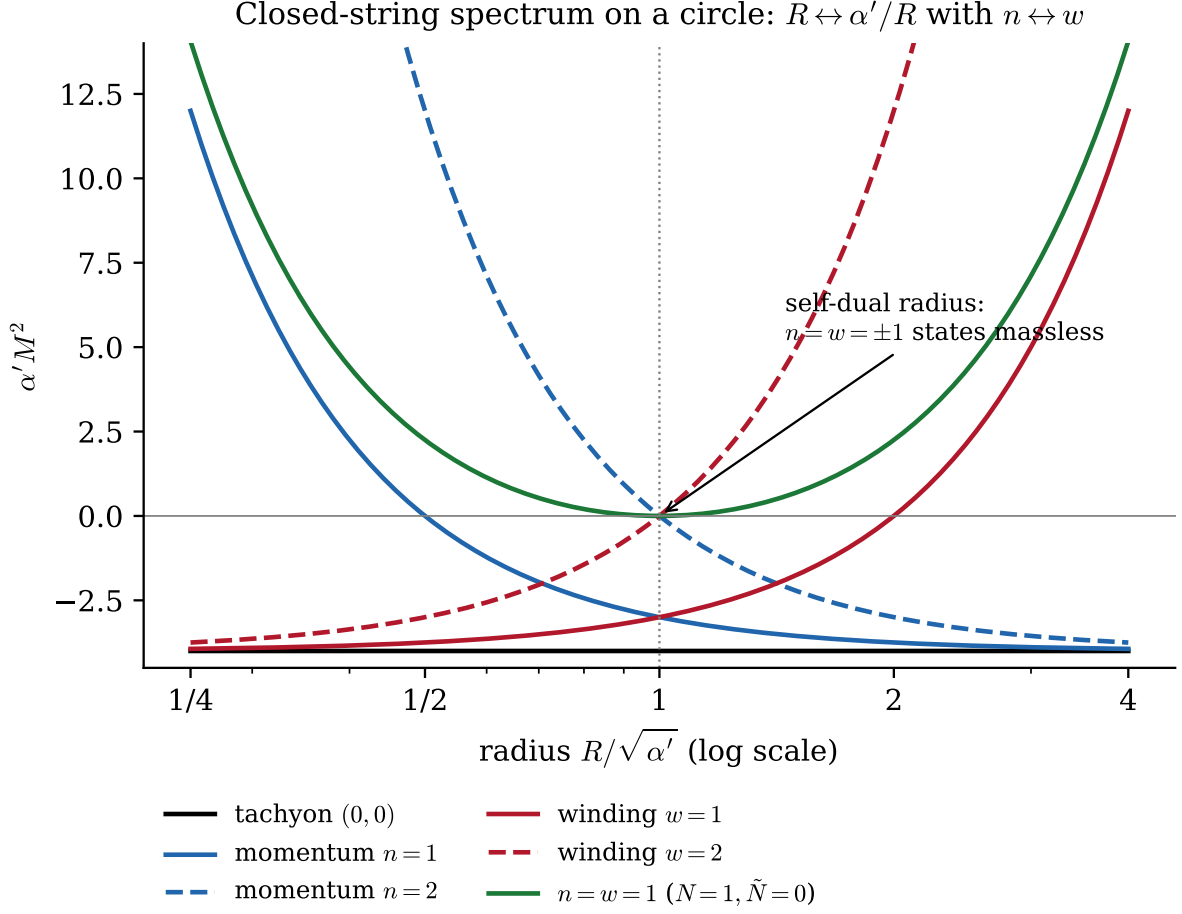
Figure 2: Lowest mass levels of the closed bosonic string on a circle of radius R as a function of \log R , with the lowest oscillator levels allowed by level matching N - \tilde{N} = nw . Momentum and winding curves are mirror images under R \mapsto \alpha'/R ; at the self-dual radius the n = w = \pm 1 states become massless (enhanced gauge symmetry). Computed figure; data: Tong §8.2, ll. 11351–11470; Lean leftMomentum , rightMomentum (units \alpha' = 1 ).
