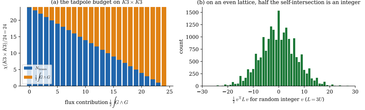
Figure 7: (a) Every way to split the tadpole budget \chi(K3 \times K3)/24 = 576/24 = 24 between space-filling branes and flux ( k3k3_anomaly , tadpole_budget ). (b) For random integer flux vectors on the even lattice 3U , \frac{1}{2}v^T L v is always an integer, the lattice fact behind flux quantization ( kronForm_even , flux_half_selfIntersection_integral ). Computed figure; data: SVW ( \chi/24 condition); DRS §2–4; Lean Flux/Tadpole.lean, Flux/Integrality.lean.
