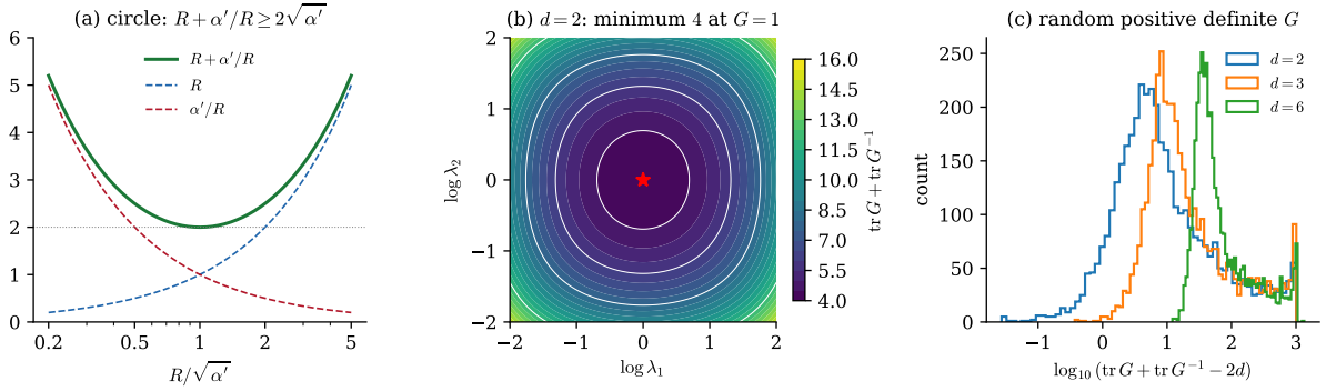
Figure 6: The dual-scale bound. (a) On a circle the effective scale R + \alpha'/R is minimized at the self-dual radius. (b) For d = 2 and positive-definite G with eigenvalues \lambda_{1,2} , \text{tr } G + \text{tr } G^{-1} = \sum_i (\lambda_i + \lambda_i^{-1}) has its minimum 2d = 4 at G = 1 . (c) Excess over 2d for 4000 random positive definite matrices in each dimension: never negative, as the Lean theorem dualScale_ge guarantees. The plot illustrates the theorem; it proves nothing. Computed figure; data: Lean dualScale_circle, circle_effective_scale_ge_two, dualScale_ge (TraceBound.lean).
