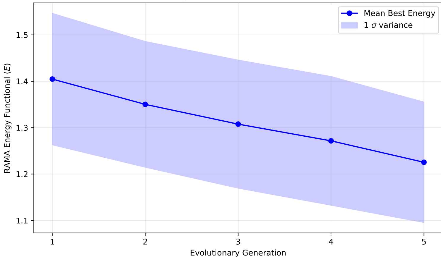
Convergence of Genetic RAMA Search
