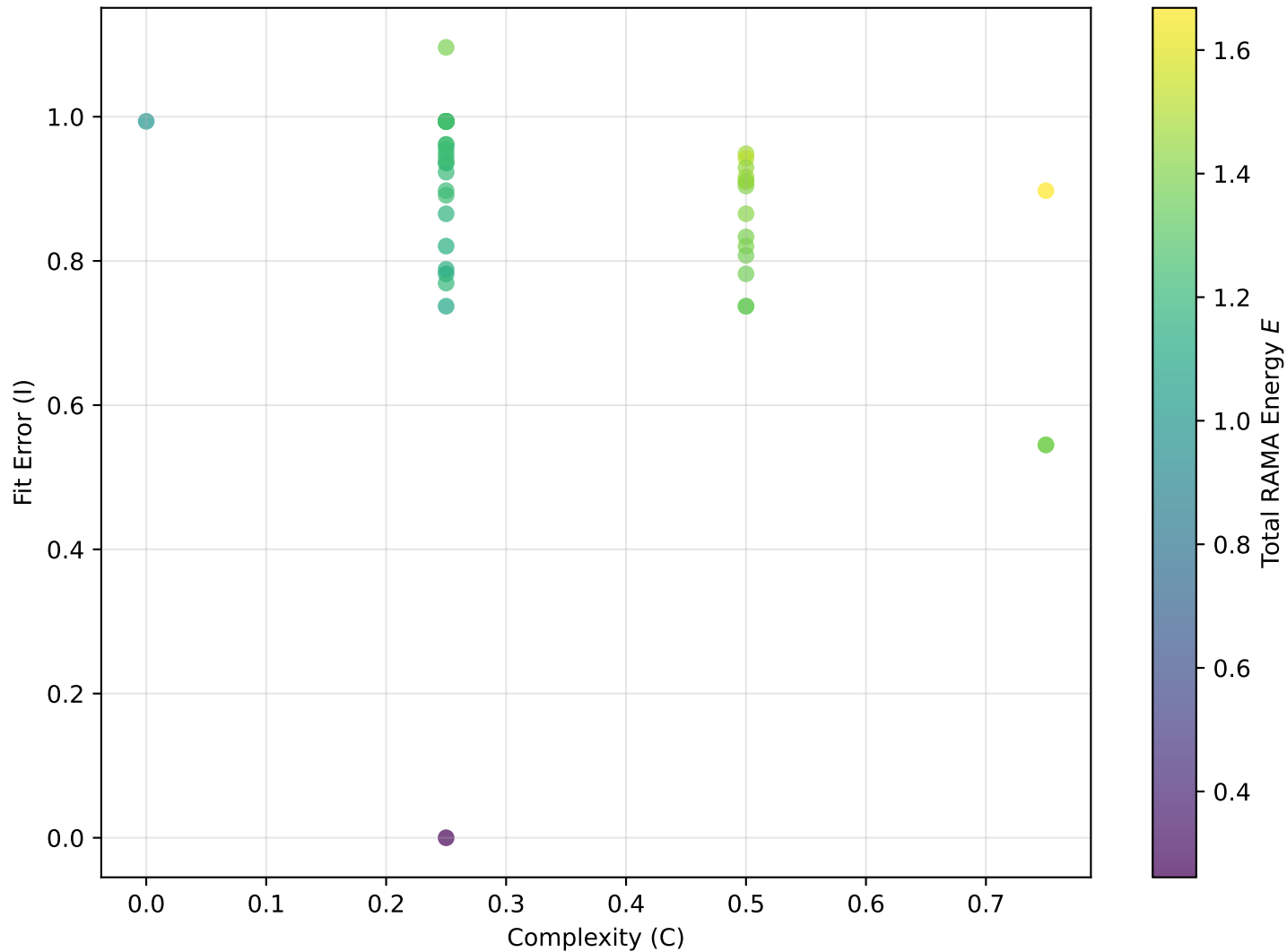
RAMA Energy Landscape: K3 \eta -quotients
