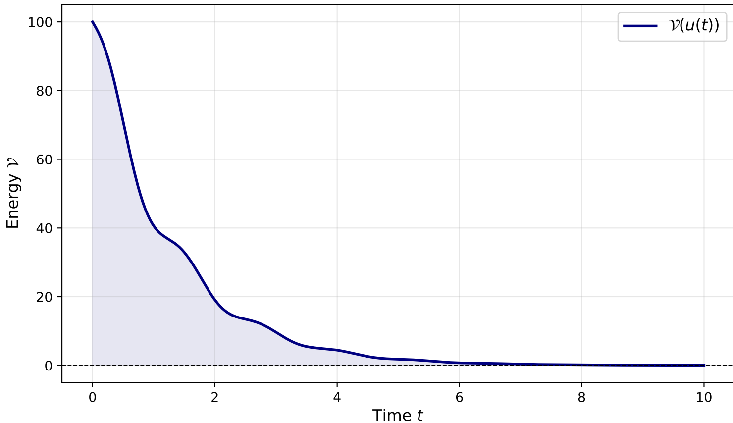
Decay of the Alien Lyapunov Functional \mathcal{V}(u)
