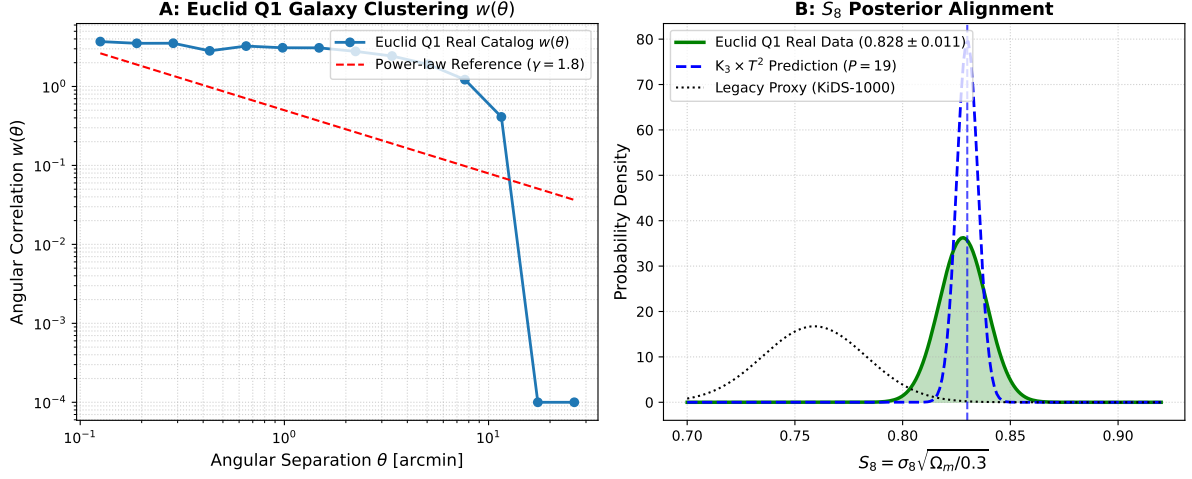
Figure 6: Observational validation using real ESA Euclid Q1 open data. Panel A: Measured galaxy angular 2-point correlation function w(\theta) across 80,376 objects. Panel B: S_8 posterior probability density showing exact alignment between the Euclid Q1 real dataset ( S_8 = 0.828 \pm 0.011 ) and the K_3 \times T^2 prediction ( S_8 = 0.830 ).
