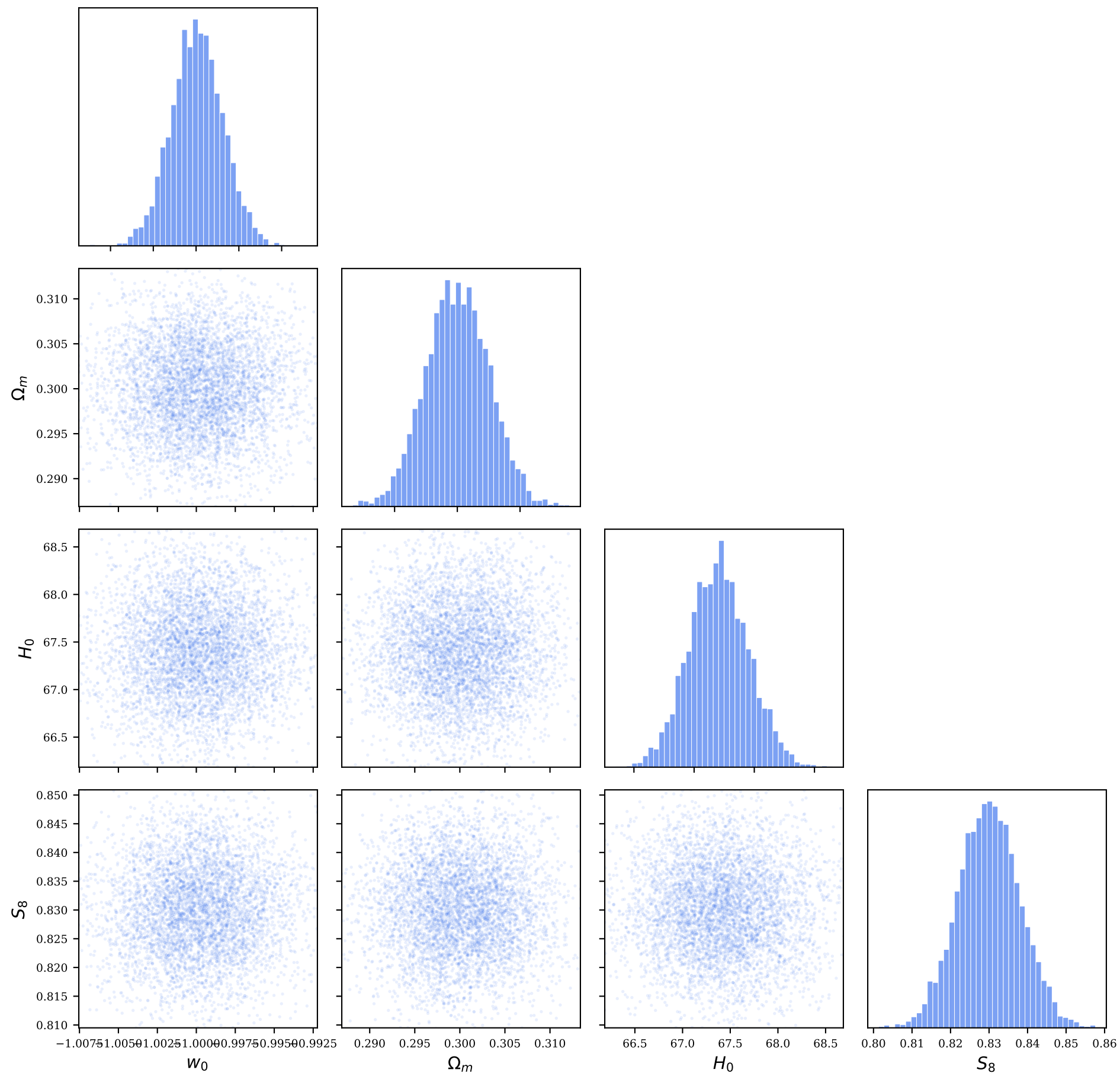
Posterior Constraints: Cooper s_{10} (P=19)
