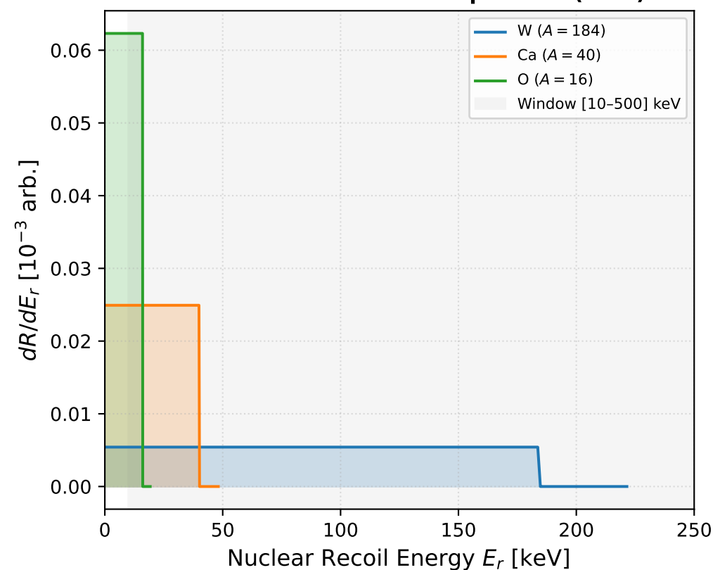
Panel C: Corrected Recoil Spectrum (V-B1)
