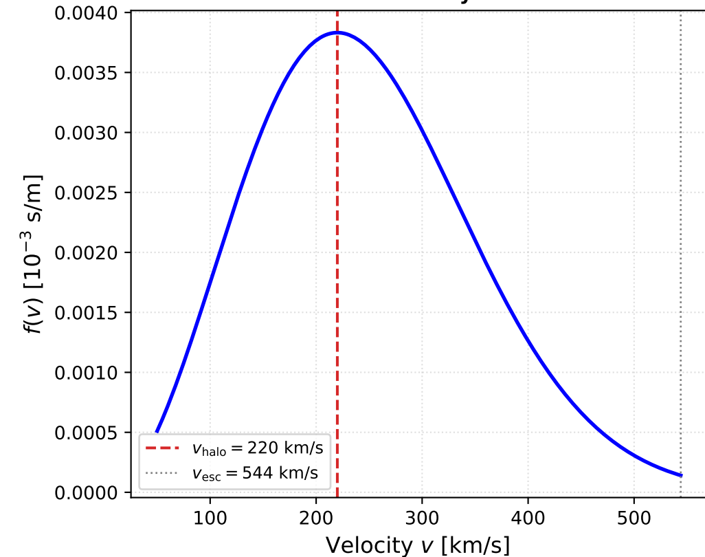
Panel A: Halo Velocity Distribution
