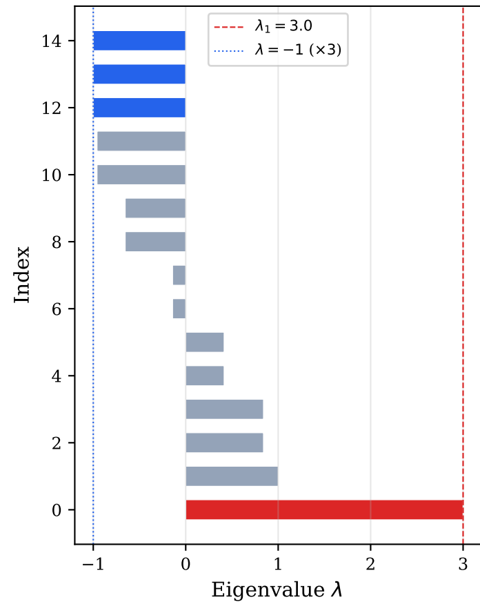
(a) Spectrum of M_{K_4 + \text{ring}}
