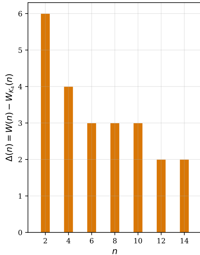
(c) Vacuum Ring Correction
