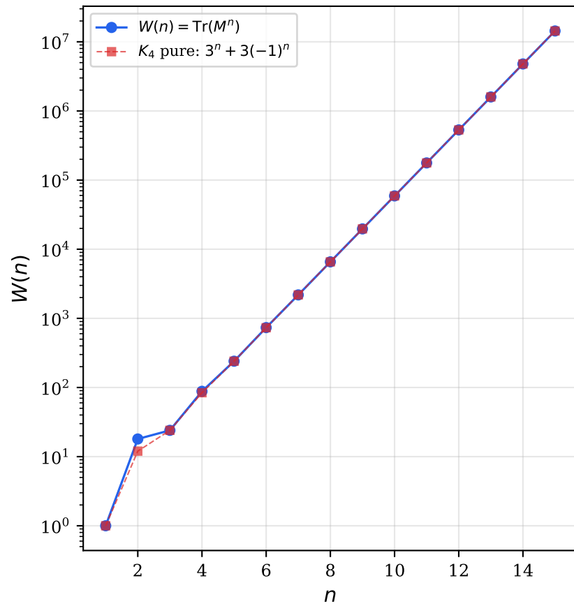
(b) Causal Loop Sequence W(n)
