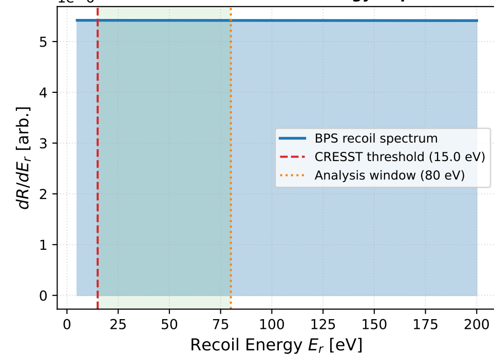
Panel C: Nuclear Recoil Energy Deposit
