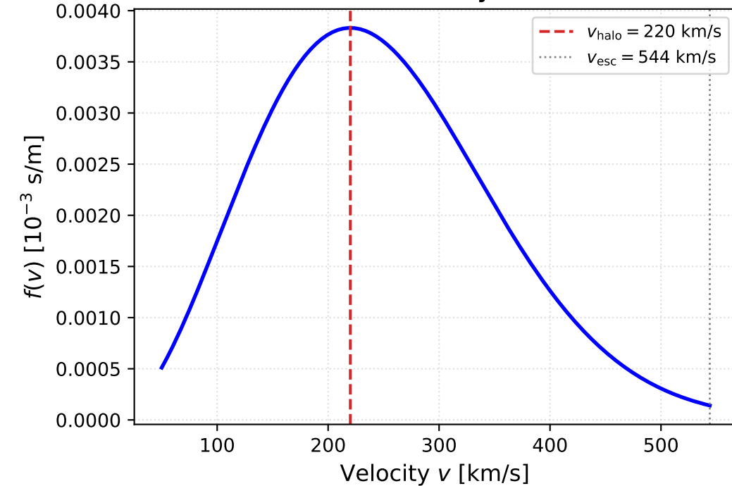
Panel A: Halo Velocity Distribution
