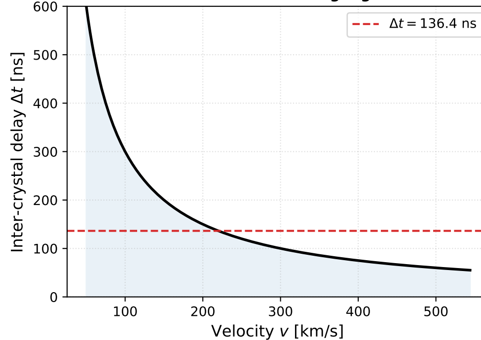
Panel B: BPS Relic Timing Signature
