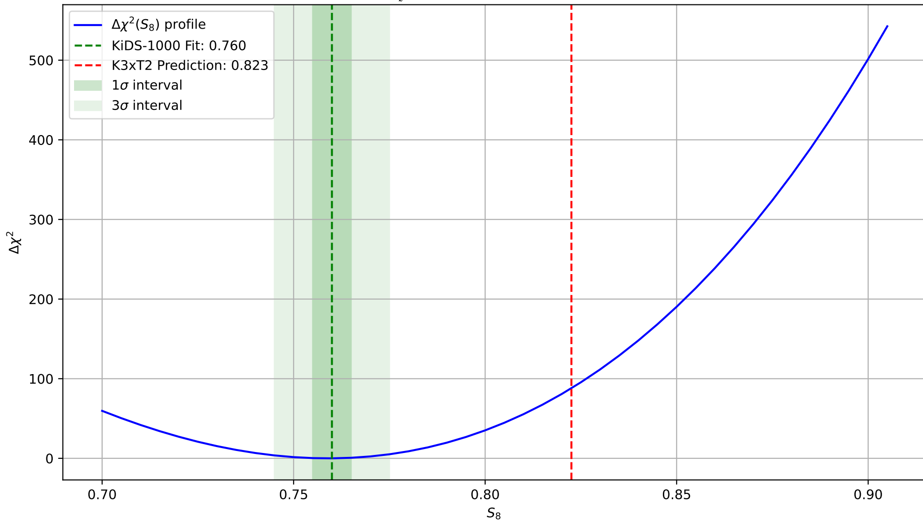
KiDS-1000 C_\ell^{EE} Band Powers: S_8 Likelihood Profile
