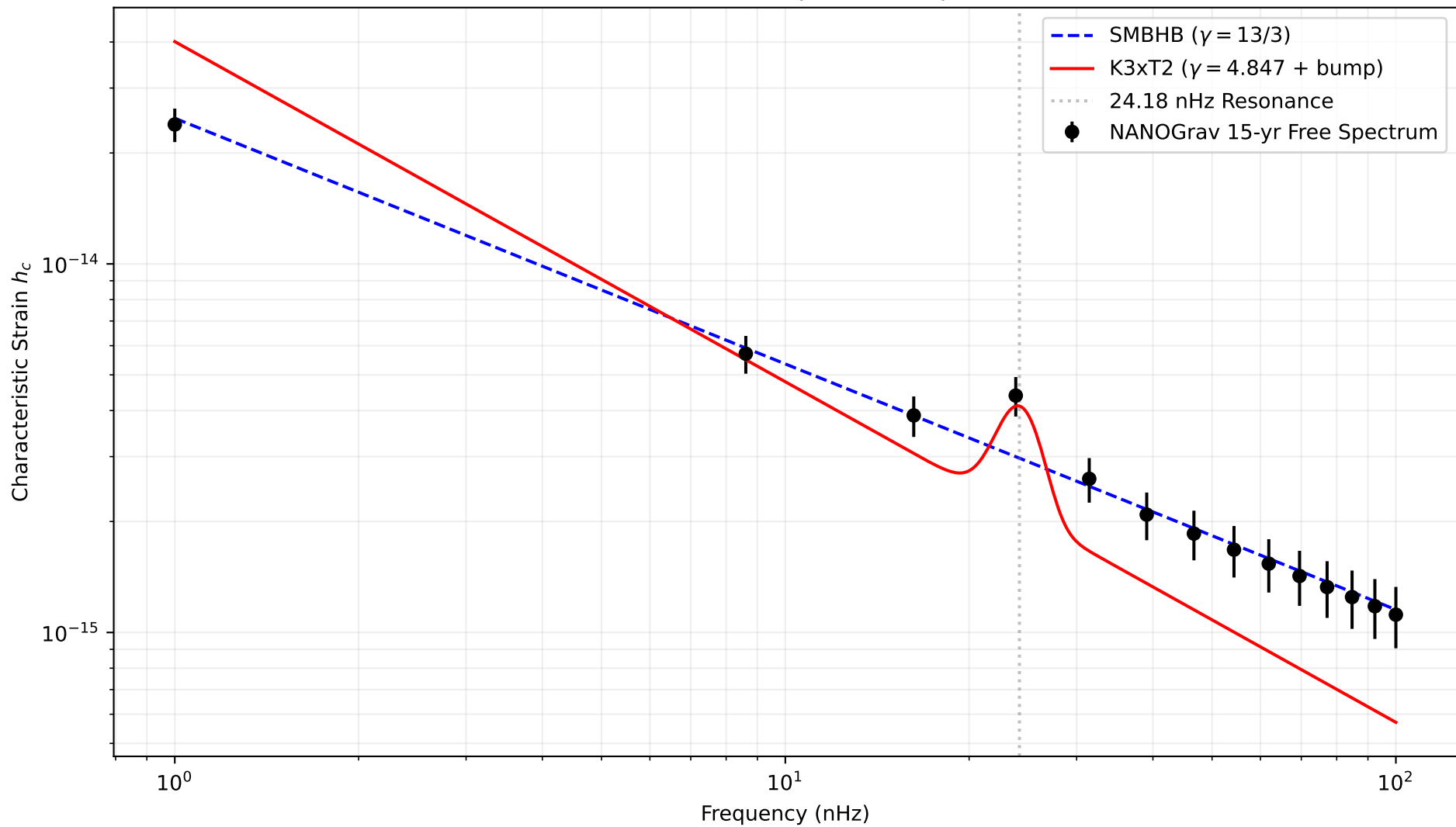
NANOGrav 15-Year Spectral Shape Test
