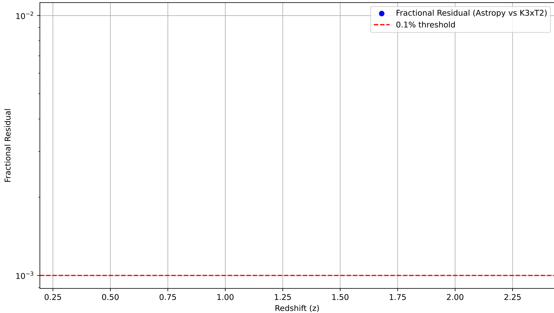
DESI BAO Distance Ladder Cross-Check: Astropy vs Trapezoidal Integrator
