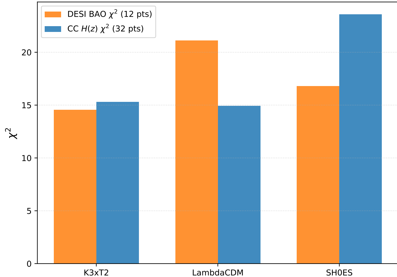
Panel B: BAO \times CC Joint \chi^2 Decomposition
