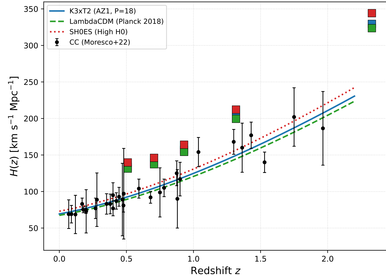
Panel A: CC H(z) + DESI D_H/r_d Overlap
