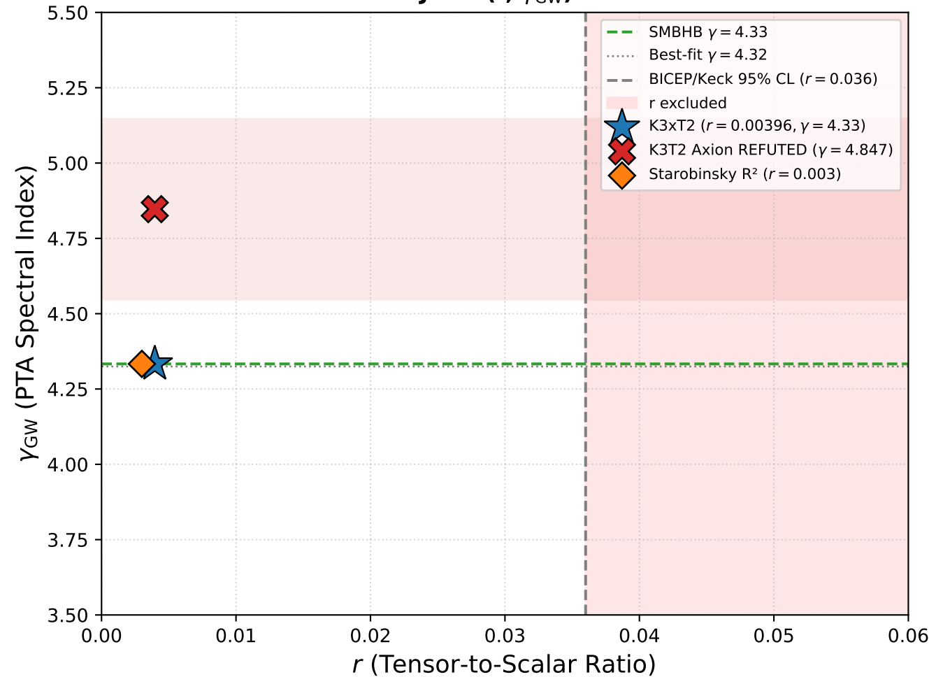
Panel B: Joint ( r , \gamma_{\text{GW}} ) Exclusion
