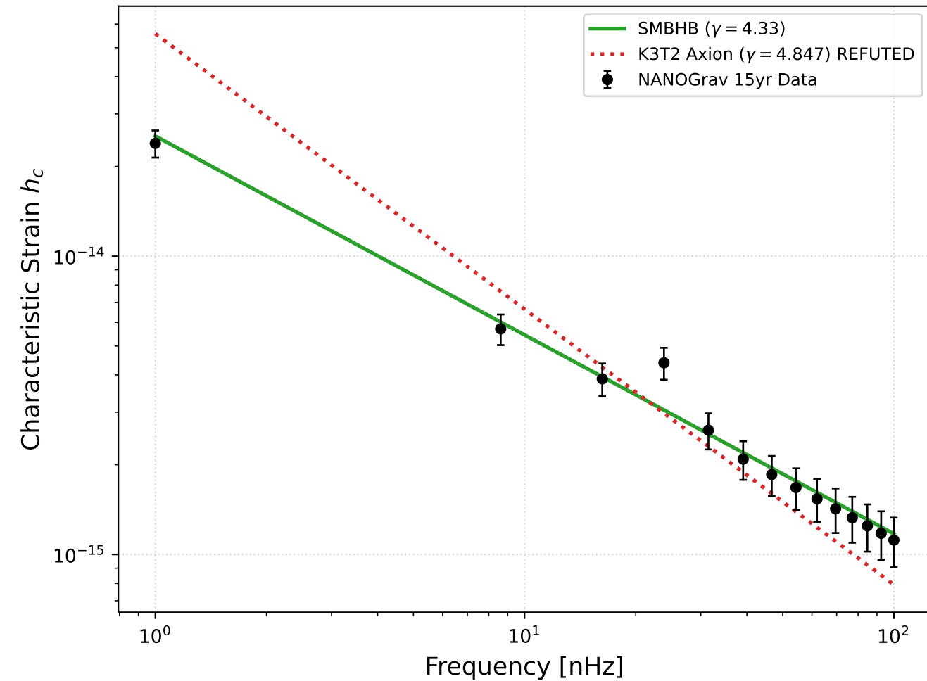
Panel A: NANOGrav 15yr Strain Spectrum
