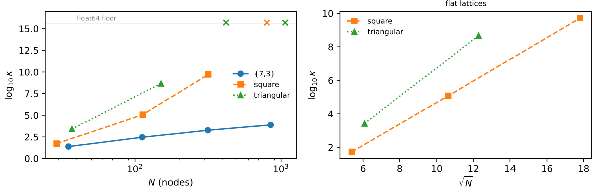
Figure 1: Left: \log_{10} \kappa of the DtN sensitivity Jacobian versus N . Filled markers are double-precision values; open markers are the ball-arithmetic values of Section 2.4 for instances that are singular in double precision (crosses at the floor where no such value is available). Right: the two flat families against \sqrt{N} , the abscissa on which the depth mechanism predicts a straight line.
