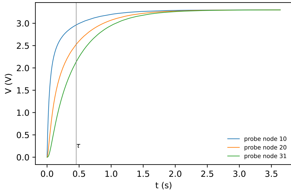
square R=6: simulated ADC record (16 bit, 860 S/s, 1 % parts)
