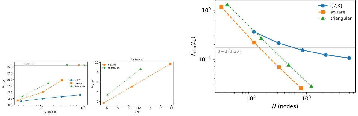
Figure 1: Left: \log_{10} \kappa of the DtN sensitivity Jacobian versus N ; crosses mark numerically singular cases, plotted at the double-precision floor. Right: Dirichlet spectral gap \lambda_{\min}(L_{ii}) of the RC network; the \{7, 3\} points at N = 2240 and 5887 are exploratory. The grey line is the upper bound 3 - 2\sqrt{2} on the bottom of the spectrum of the infinite \{7, 3\} graph.
