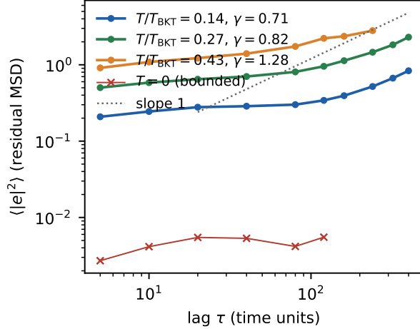
Figure 2: Mean-square residual displacement of a tracked vortex about the two-coefficient fit, against lag, at the three temperatures and at T = 0 (log-log). The local exponents over lags 20–400 are 0.71, 0.82 and 1.28; over lags \geq 100 the two cooler temperatures give 1.1–1.2. The T = 0 curve is bounded (sound).
