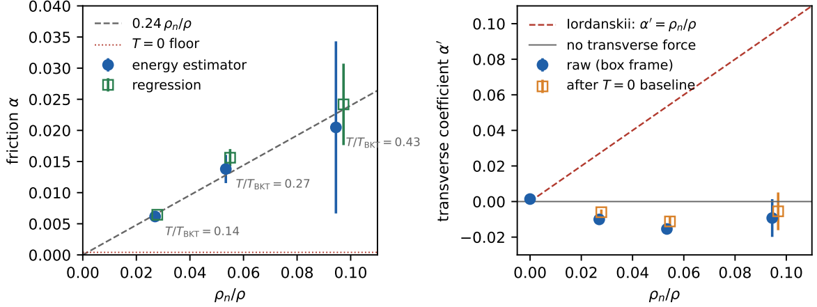
Figure 1: Left: friction \alpha against the normal fraction \rho_n/\rho of the base state, from the energy estimator (2) and from the trajectory regression, with the line \alpha = 0.24 \rho_n/\rho and the T = 0 floor of the instrument. Right: transverse coefficient \alpha' as measured in the box frame (circles) and after subtracting the T = 0 kinematic baseline of a compressible pair at the sizes the fits use (squares), against the Iordanskii prediction \alpha' = \rho_n/\rho and the no-transverse-force value 0. Errors are block jackknives over runs.
