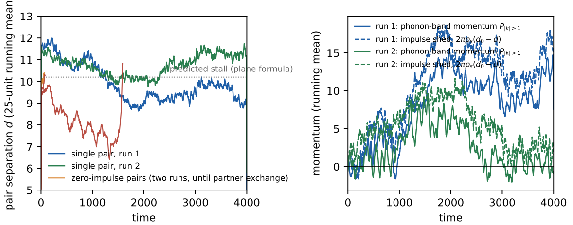
Figure 3: Left: separation of two single pairs ( d_0 = 12 , T/T_{\text{BKT}} = 0.14 , L = 64 , 4000 time units, 25-unit running mean) and of the zero-impulse pairs of the same temperature until their partner exchange. Right: the momentum of the modes with |k| > 1 projected on the pair’s initial impulse, against the impulse shed by the pair, 2\pi\rho_s(d_0 - d) .
