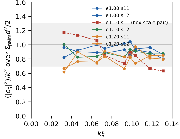
Figure 5: Vortex-charge structure factor of the six equilibrated L = 192 states, \langle |\rho_q(k)|^2 \rangle / k^2 on the shells |m|^2 = 1\text{--}16 , divided by the dipole polarisability \Sigma_{\text{pairs}} d^2 / 2 computed from the minimum-cost matching of the detected vortices; the band is the registered \pm 30\% . The dashed run still carries a box-scale pair.
