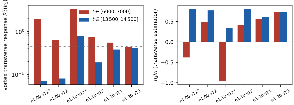
Figure 4: The six L = 192 trajectories at two sampling windows, t \in [6000, 7000] and, after continuing them, t \in [13500, 14500] : the vortex-driven transverse response at the longest wavelength (left, logarithmic; the dotted line is the registered threshold 0.45) and the superfluid fraction from the transverse estimator (right). Starred runs are the two that had a negative superfluid fraction.
