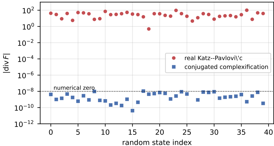
Phase-space divergence (N=6)
