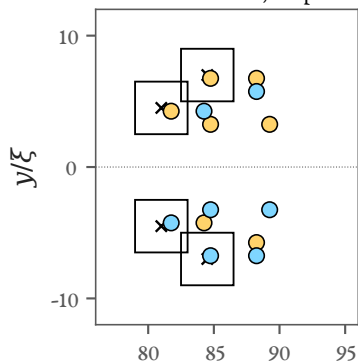
b t = 40 \tau : 4 counted, 14 present
