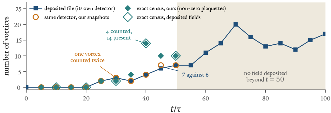
b t = 40 \tau : 4 counted, 14 present
