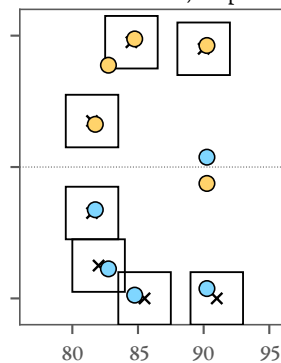
c t = 50 \tau : 7 counted, 10 present
