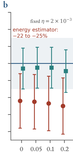
Panels a, b: Rust example g0_scan, 8 seeds of 8 tracks (nominally 2000 time units), mean \pm standard deviation over seeds; rusty-SUNDIALS commit 5db8041. Panel c: the registered tracks (numpy seed 20261005), analysed by both implementations.
