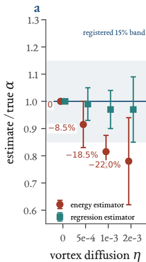
Panels a, b: Rust example g0_scan, 8 seeds of 8 tracks (nominally 2000 time units), mean \pm standard deviation over seeds; rusty-SUNDIALS commit 5db8041. Panel c: the registered tracks (numpy seed 20261005), analysed by both implementations.
