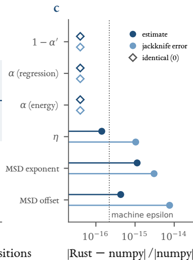
Panels a, b: Rust example g0_scan, 8 seeds of 8 tracks (nominally 2000 time units), mean \pm standard deviation over seeds; rusty-SUNDIALS commit 5db8041. Panel c: the registered tracks (numpy seed 20261005), analysed by both implementations.
