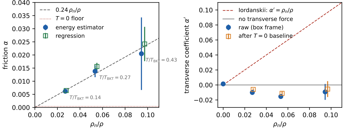
Figure 2: Left: friction \alpha against the normal fraction \rho_n/\rho of the base state, from the energy estimator (2) and from the trajectory regression, with the line \alpha = 0.24 \rho_n/\rho and the T = 0 floor of the instrument. Right: transverse coefficient \alpha' as measured in the box frame (circles) and after subtracting the T = 0 kinematic baseline of a compressible pair at the sizes the fits use (squares), against the Iordanskii prediction \alpha' = \rho_n/\rho and the no-transverse-force value 0. Errors are block jackknives over runs.
