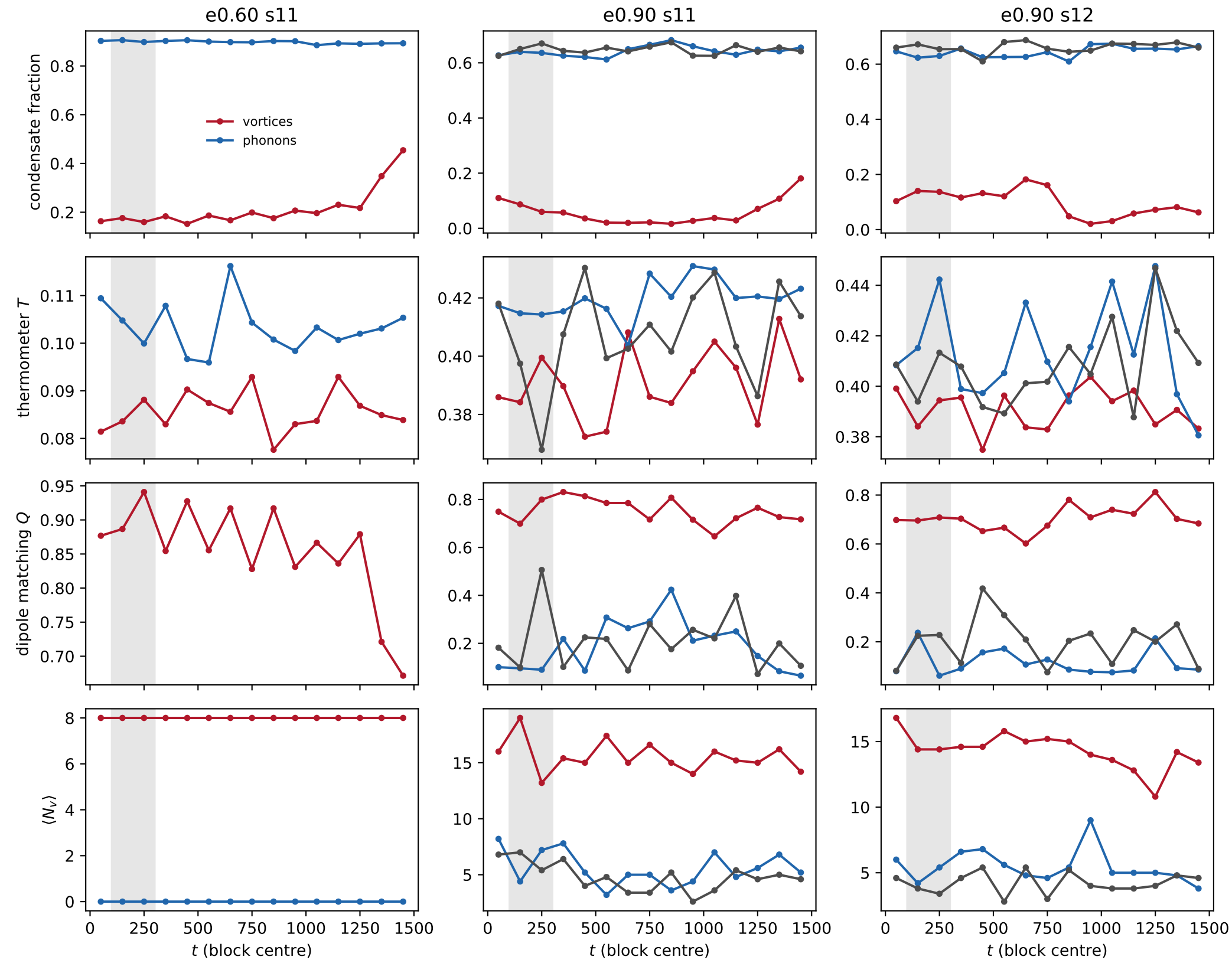
Round 2, Part I: the same energy as vortices (V) or phonons (P); shaded = pre-registered window
