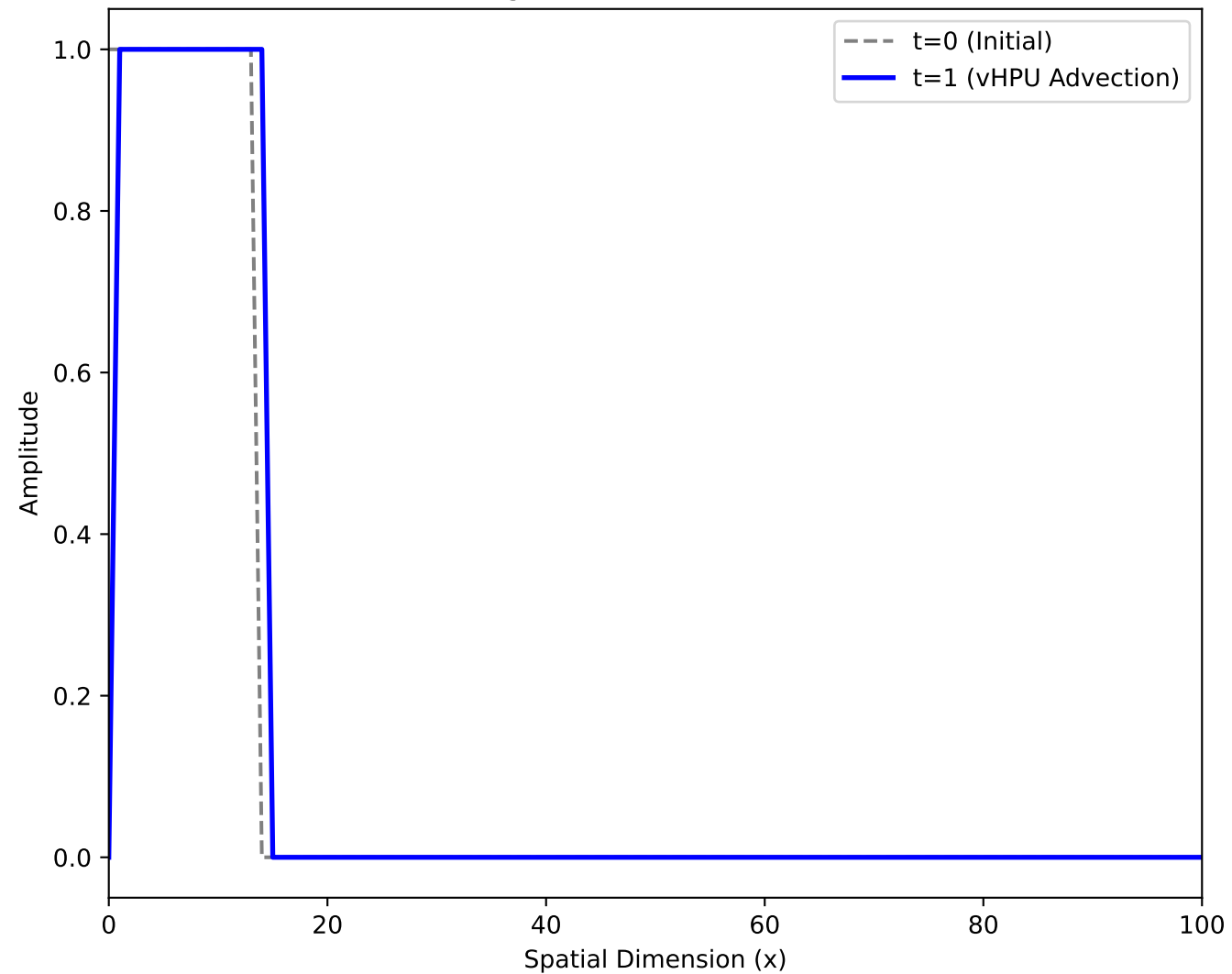
1D Burgers' Shockwave Advection
