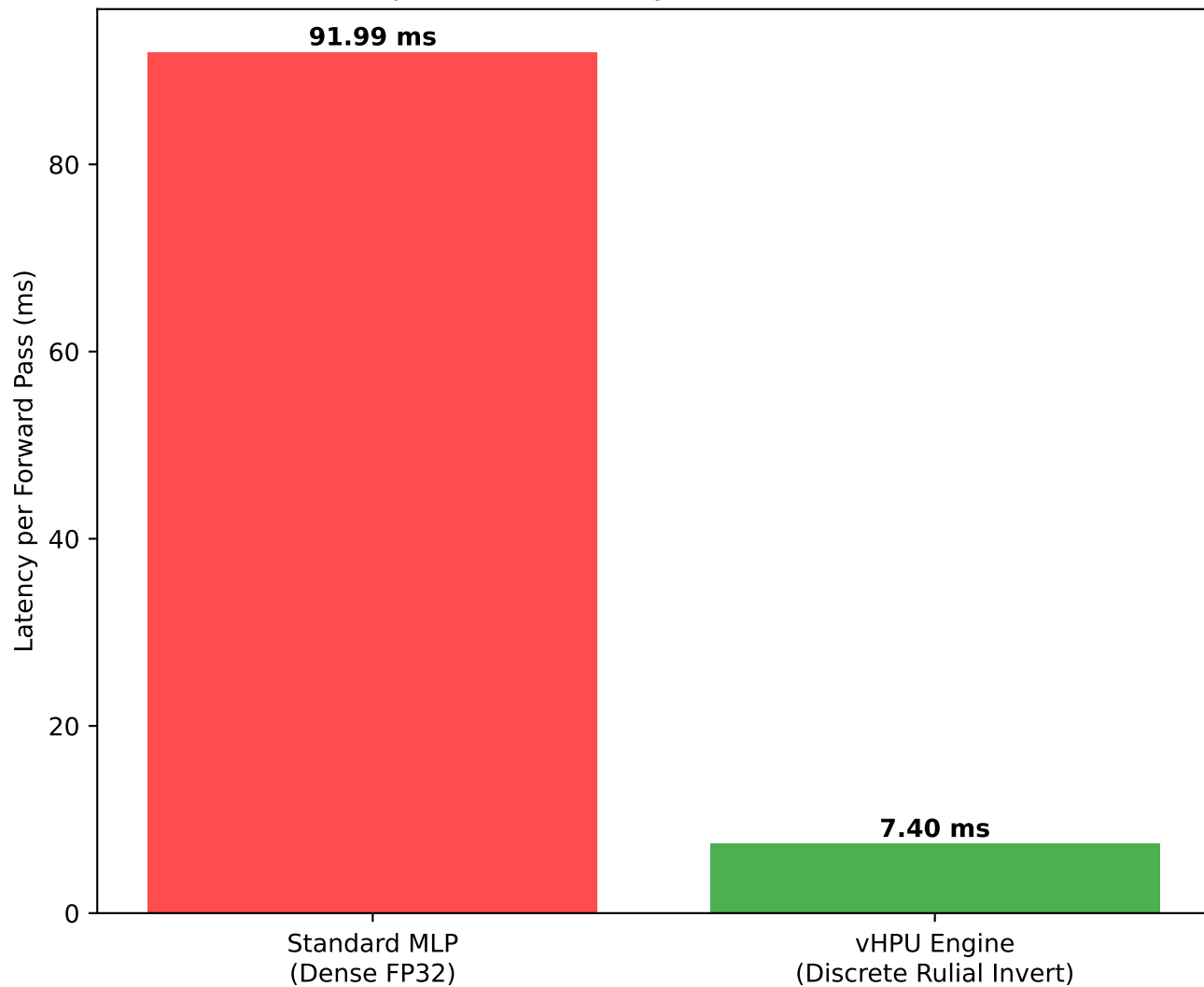
Computational Latency (Virtual Heat Profile)
