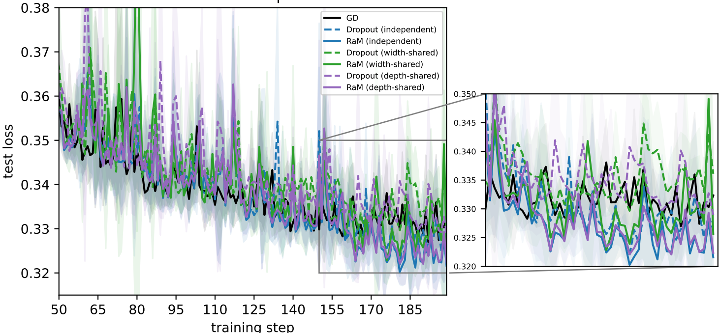
Test loss comparison
