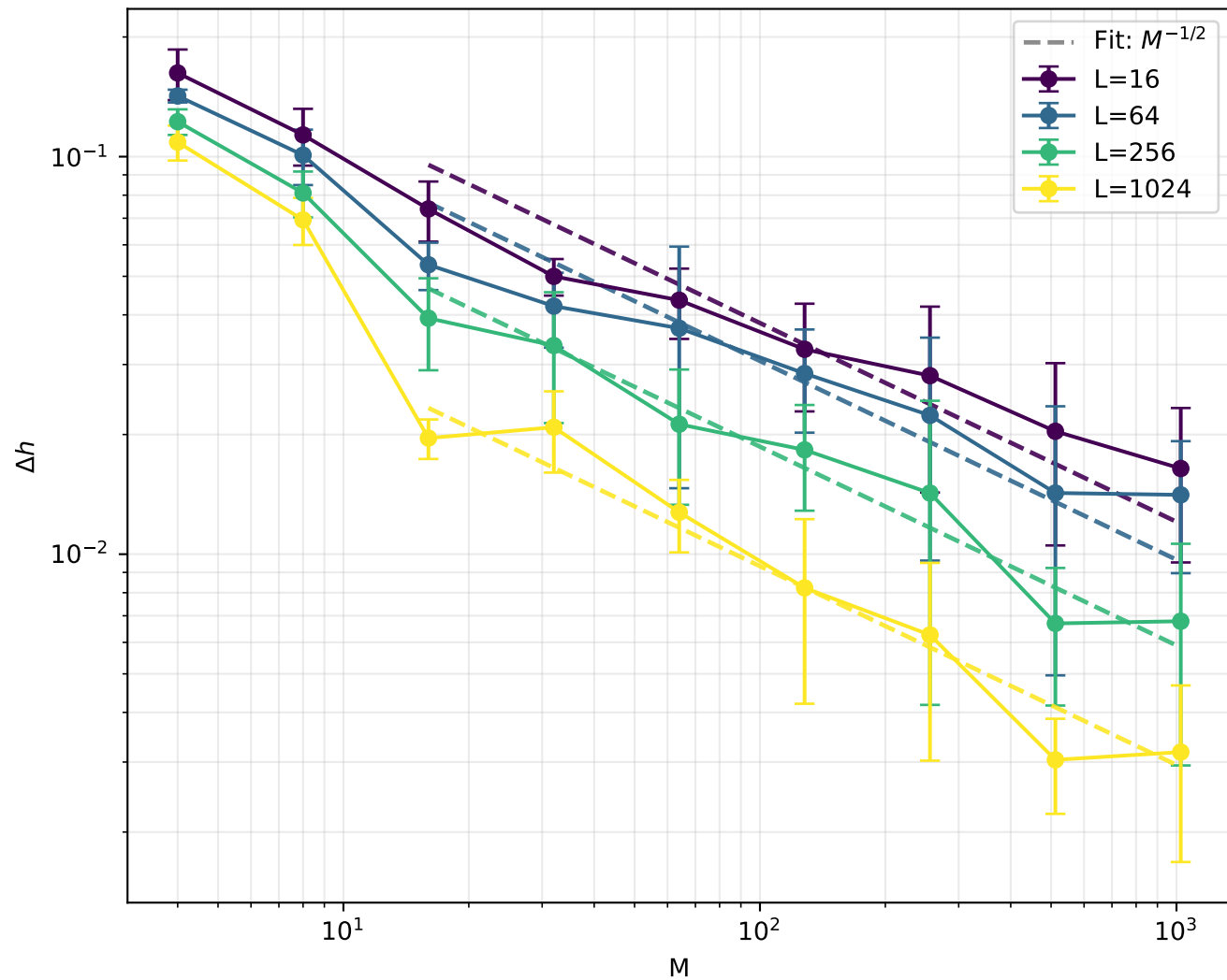
independent: \Delta h vs M (by L)
