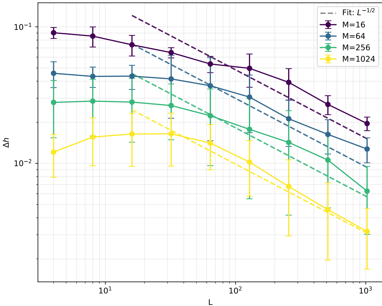
independent: \Delta h vs L (by M)
