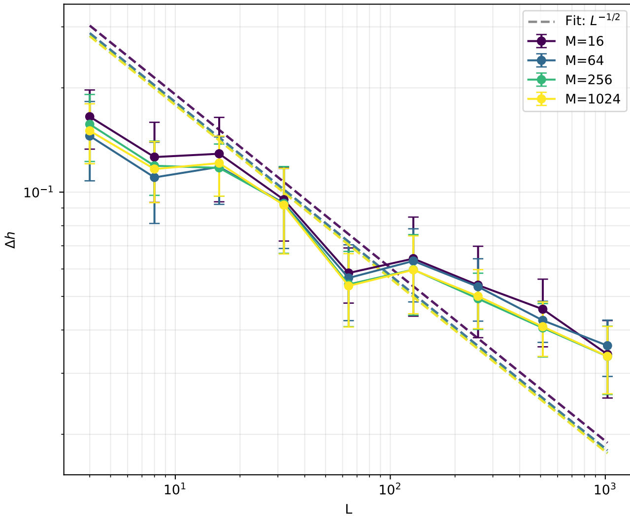
width-shared: \Delta h vs L (by M)
