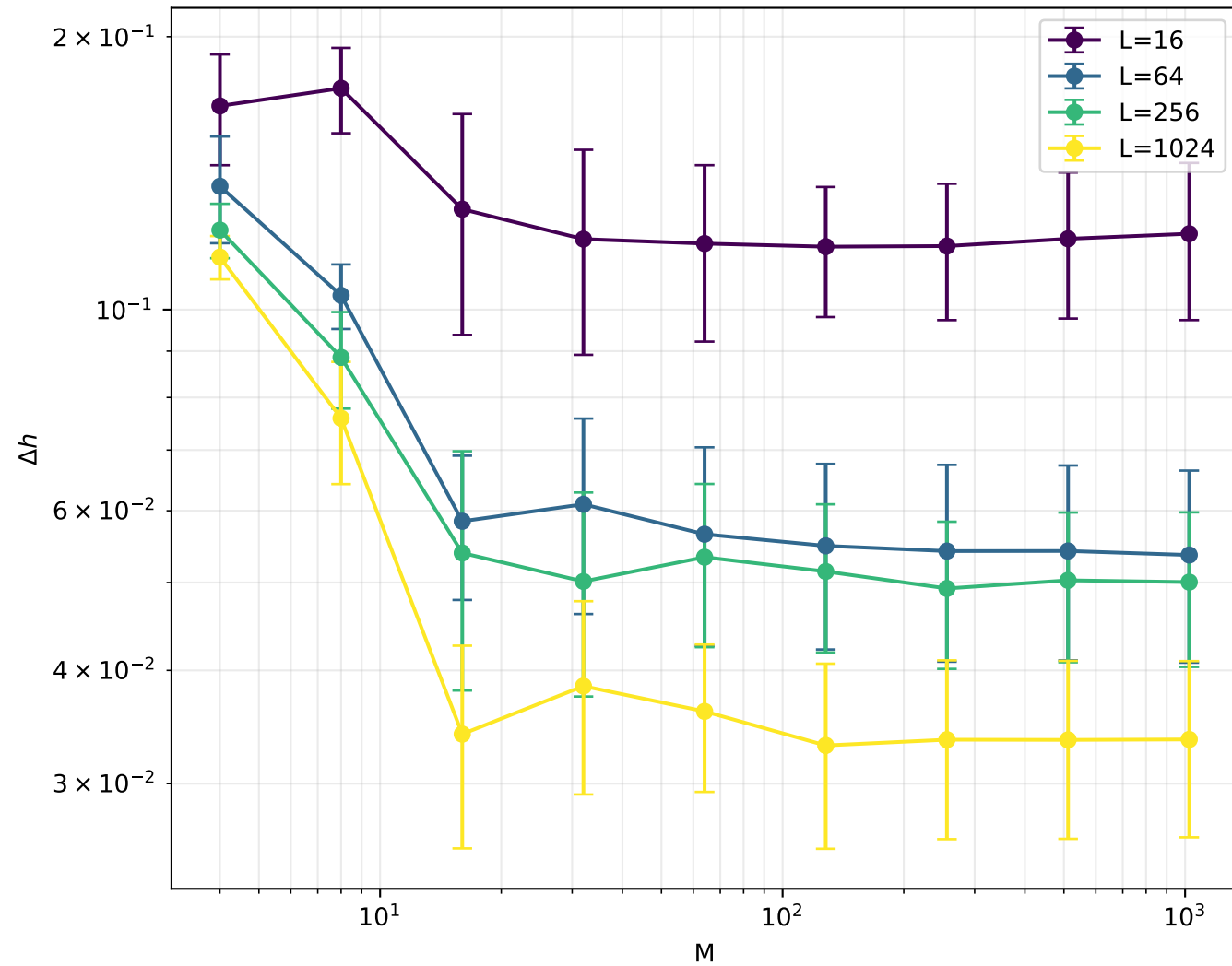
width-shared: \Delta h vs M (by L)
