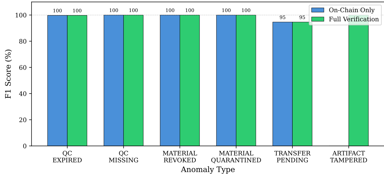
Detection Accuracy by Anomaly Type
