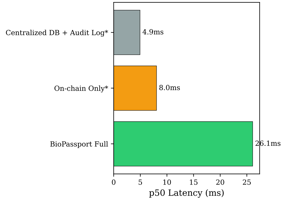
Latency Comparison
