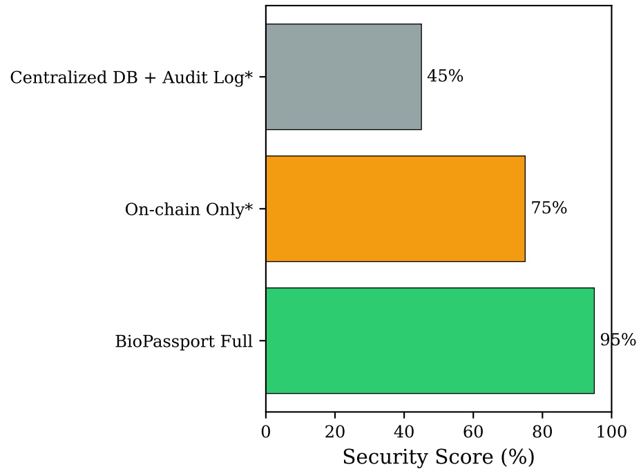
Security Comparison
