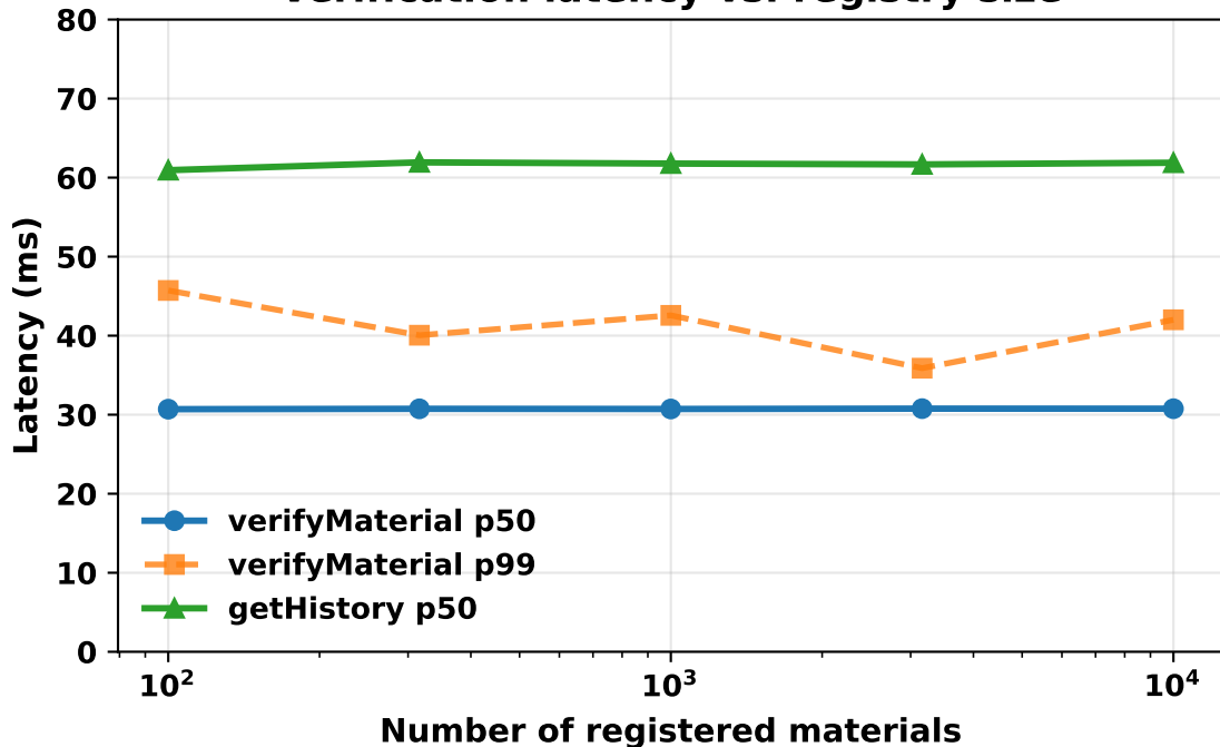
Verification latency vs. registry size
