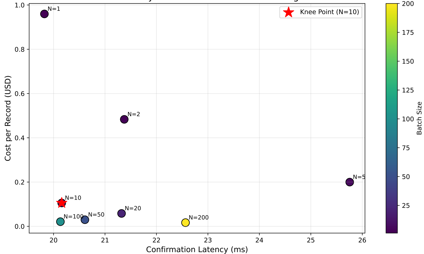
Cost-Latency Trade-off for Batched Anchoring
