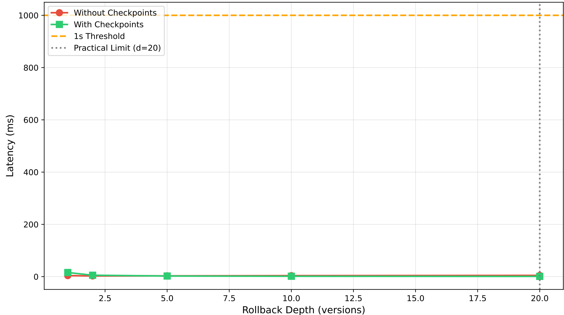
Rollback Latency vs Depth (Eq. 42)
