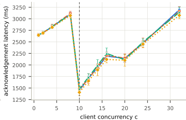
(b) acknowledgement latency
