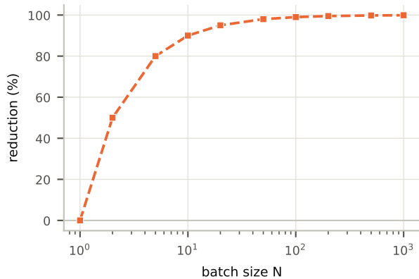
(b) reduction relative to single-record anchoring
