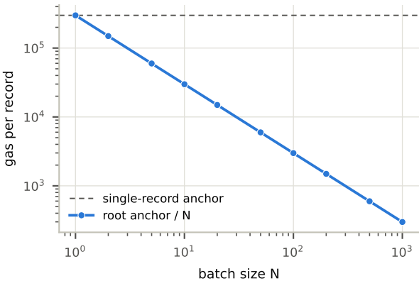
(a) amortised gas per record
