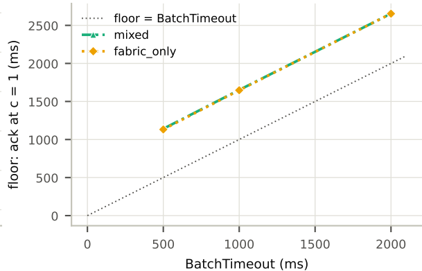
(a) transition at c = \text{MaxMessageCount} (dashed: prediction) (b) sub-threshold floor tracks BatchTimeout
