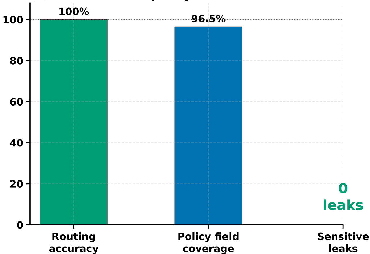
(a) Deterministic policy — 13 curated records
