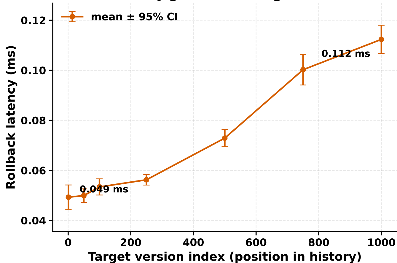
(a) Rollback latency grows with target index — NOT O(1)
