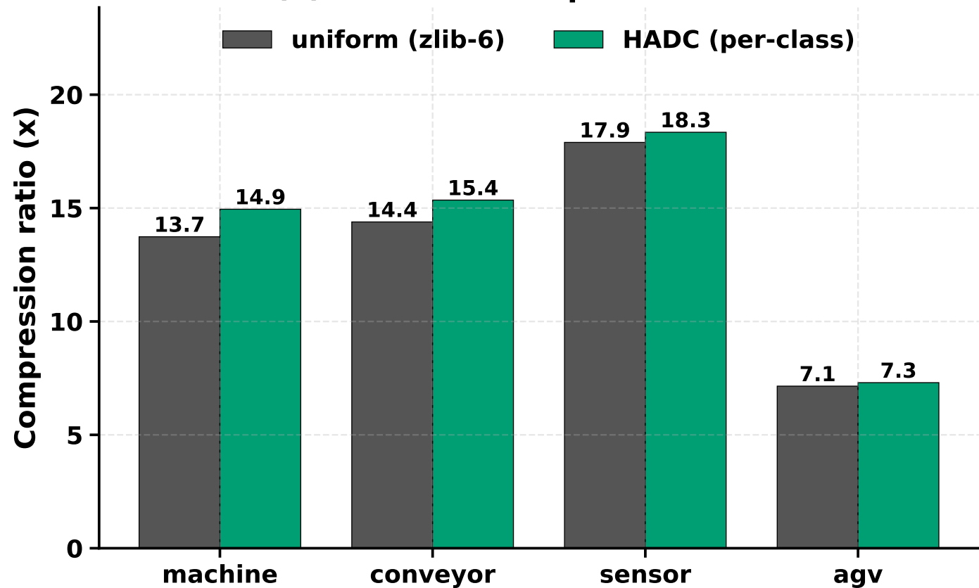
(a) Per-class compression ratio
