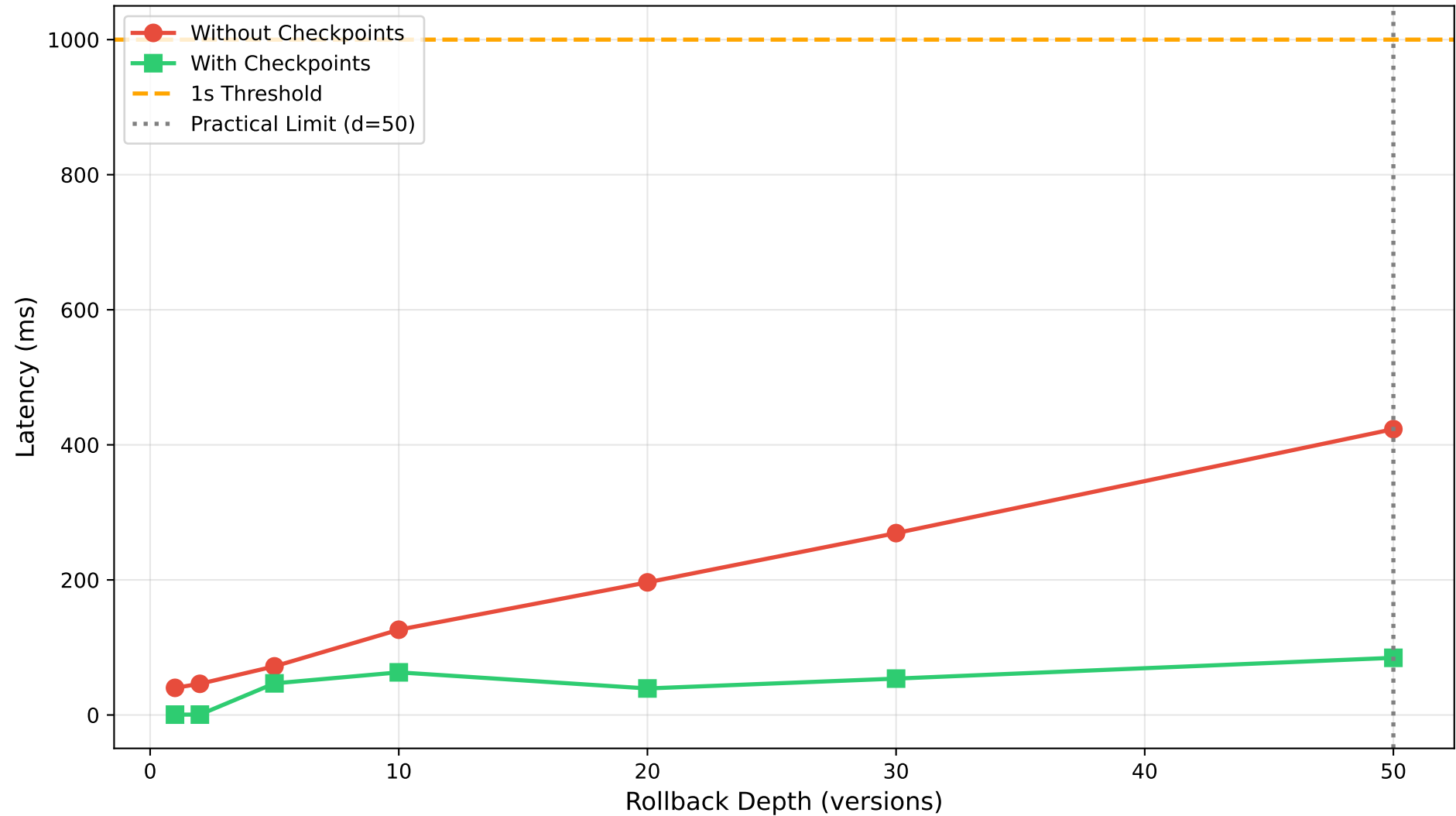
Rollback Latency vs Depth (Eq. 42)
