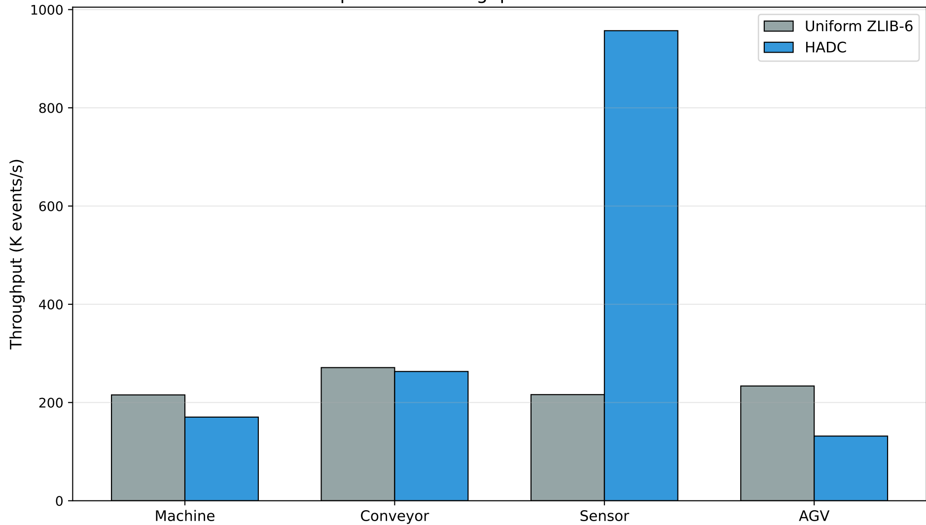
Compression Throughput: Uniform vs HADC
