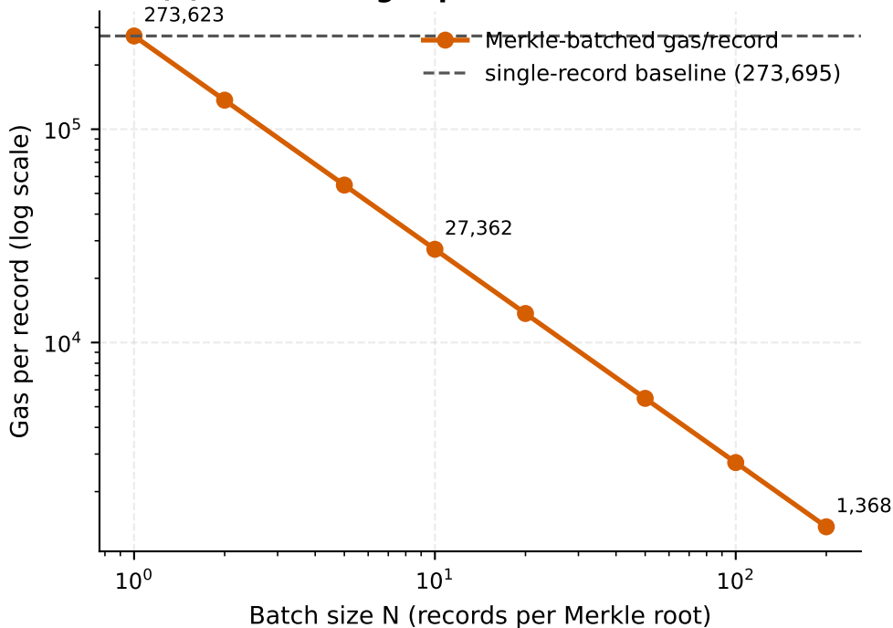
(a) Amortized gas per record vs batch size
