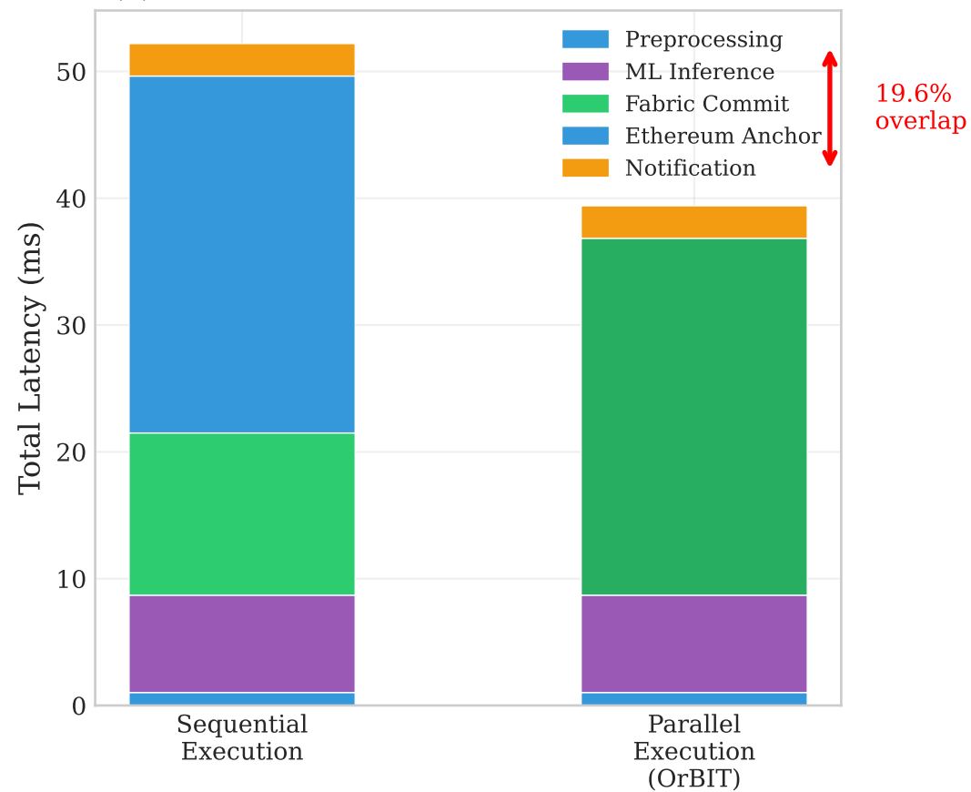
(c) Parallelization Gain: Runtime Breakdown
