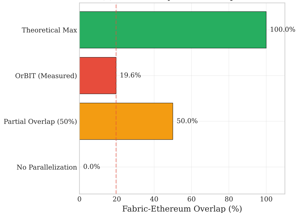
(c) Concurrency Benefit Comparison
