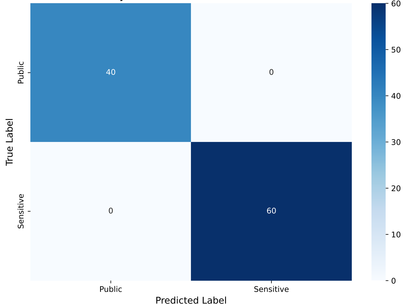
Privacy Classification Confusion Matrix
