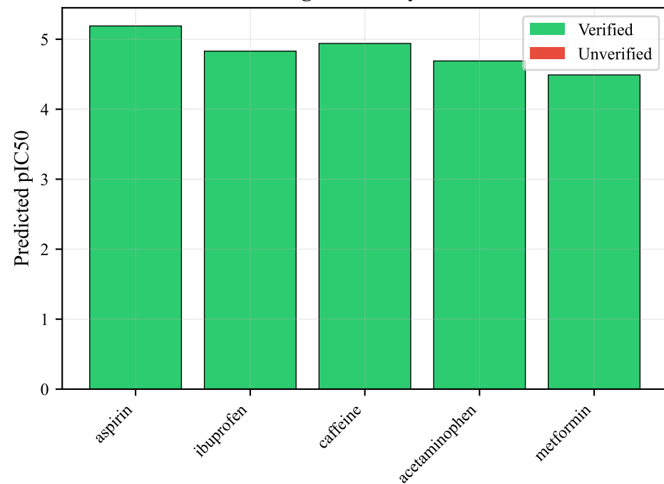
Screening Results by Molecule
