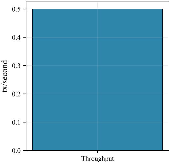
Blockchain Performance
