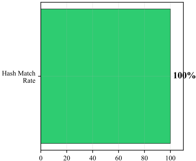
Reproducibility
