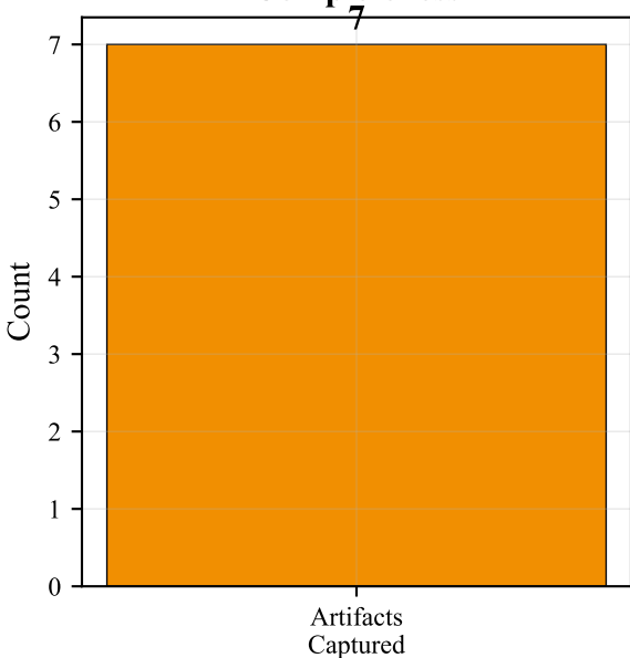
Provenance Completeness
