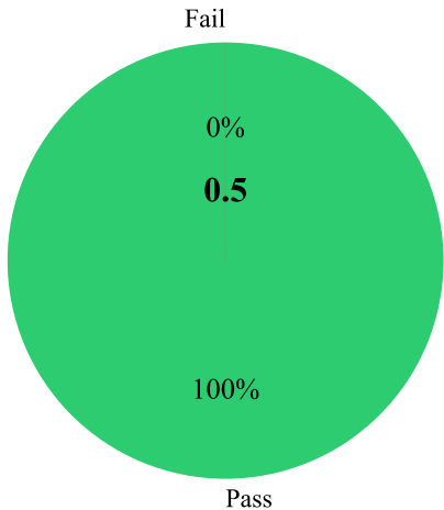
Context-Awareness Validation
