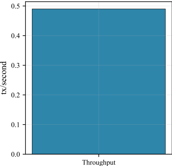
Blockchain Performance
