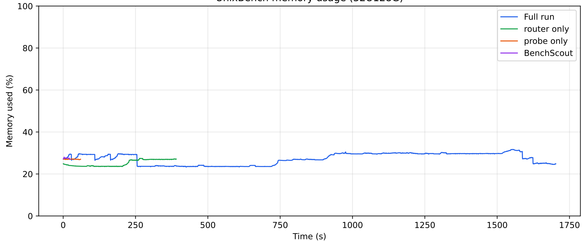
UnixBench memory usage (32U128G)
