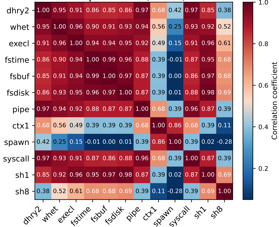
Spearman (n=25)
